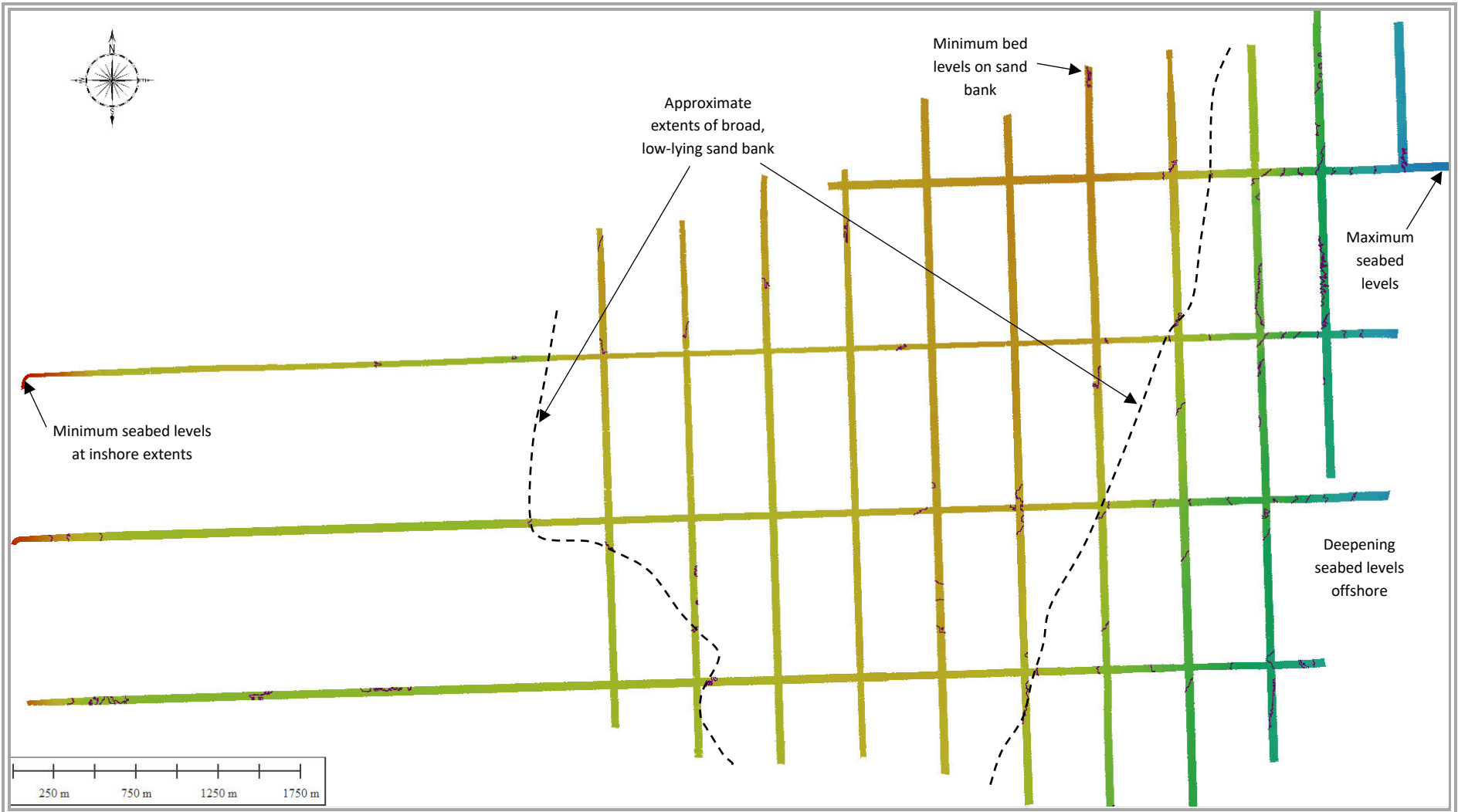
Figure 6: Bathymetric Summary (inshore survey)
